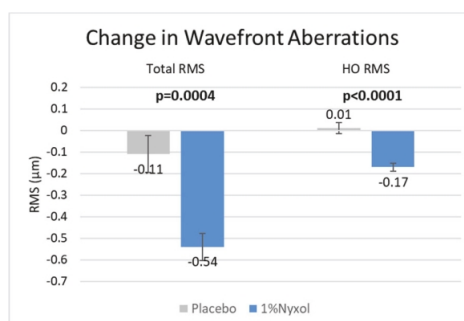
FIGURE 10. Change in Total and Higher Order (HO) Wavefront Aberrations (NYX-SNV)
